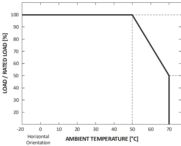
DERATING CURVE
